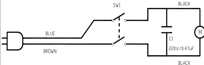
Wiring diagramme for LSU135 & LSU155 (Figure7)
